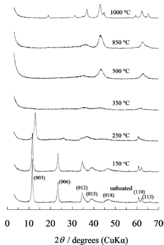
Figure 4. XRD of MgAlCO 3 formed between room temperature and 1000 °C [94].
