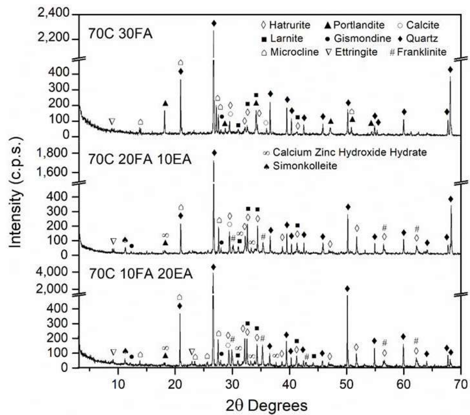
Figure 8. Mineralogical phases in 70C 30FA, 70C 20FA 10 EA and 70C 10FA 20EA SCM mixes at 28 days of curing.
